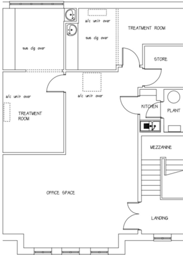
PLAN AT SECOND FLOOR LEVEL AS EXISTING
